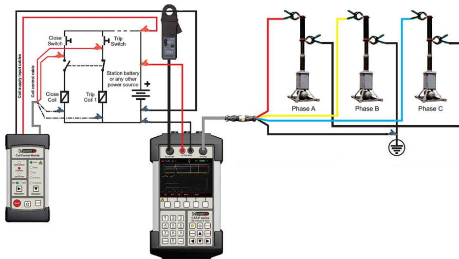
Figure 3. CAT-P and Coil Control Module connection to live tank circuit breaker with one breaking element per phase for Offline testing
