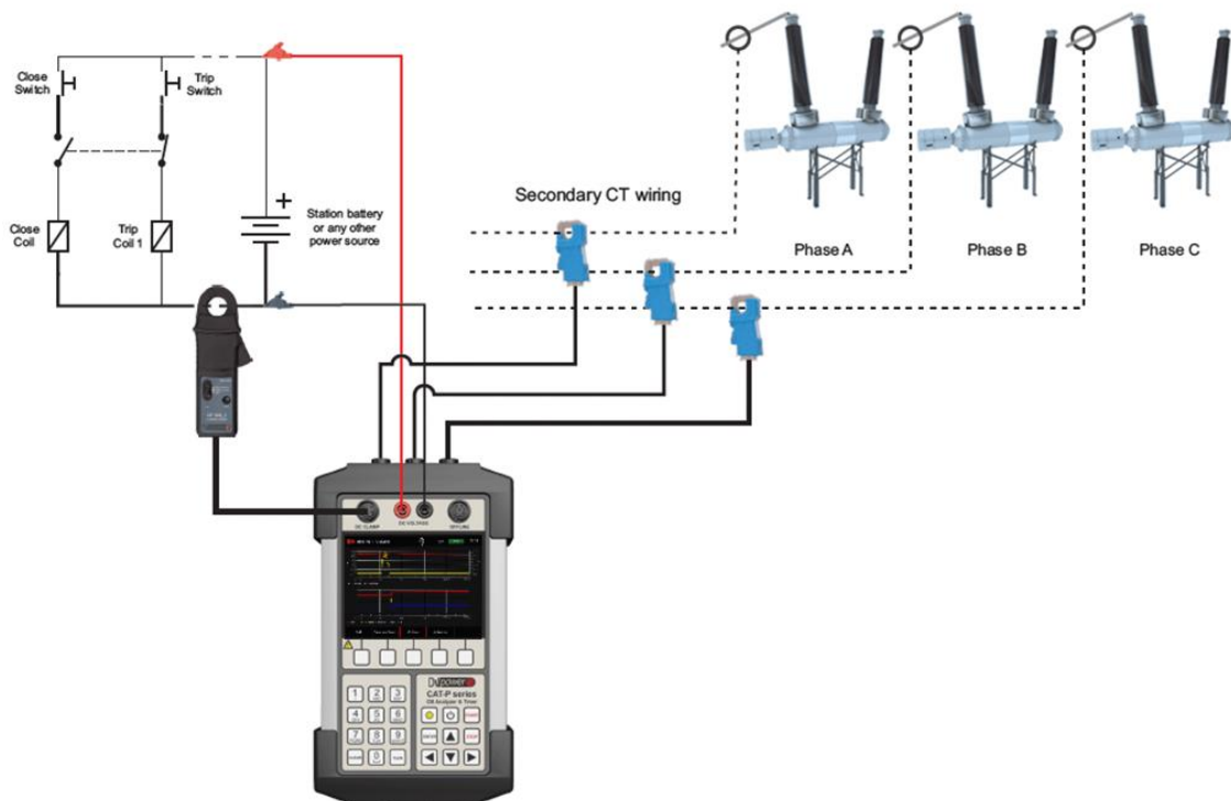
Figure 2. CAT-P connection to dead tank circuit breaker with one breaking element per phase for Online testing
